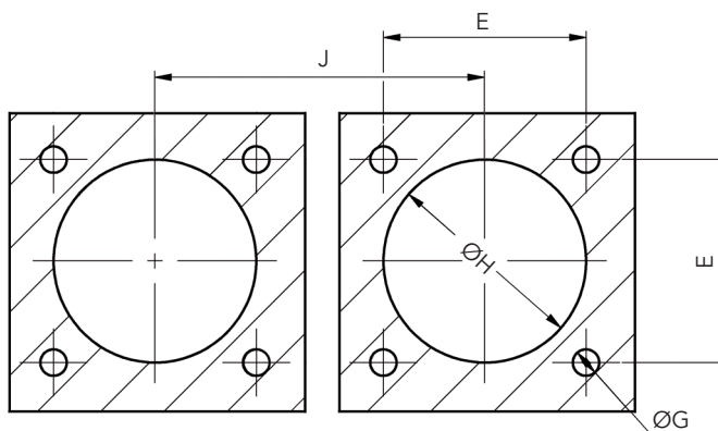
Panel cut-out
