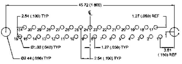
31 CONTACTS - VIEW A
