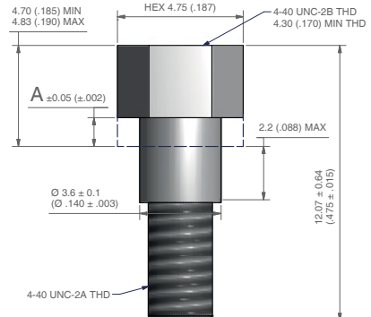
KIT PART NUMBER: MDAHMSLP1x Hardware code: Px
