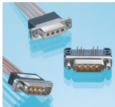
▲ COMBO MICRO-D WITH Ø2.2MM CONTACT
