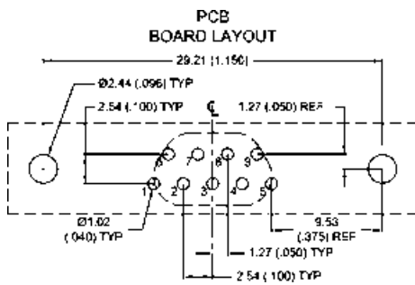
9 CONTACTS - VIEW A
