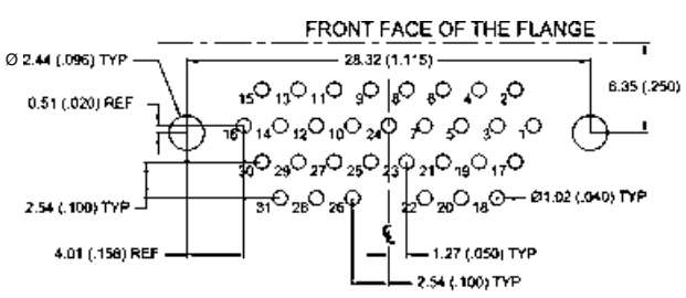
31 CONTACTS - VIEW B
