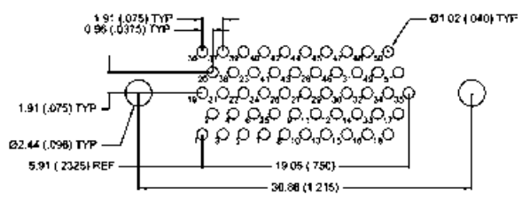
51 CONTACTS - VIEW A
