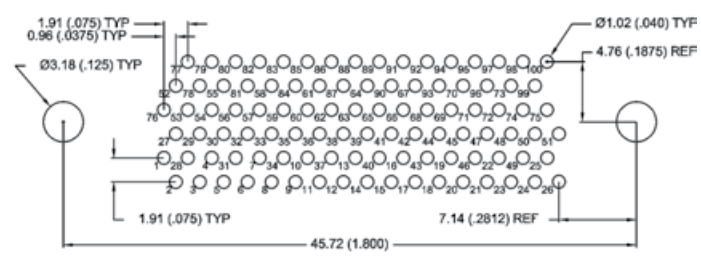
100 CONTACTS - VIEW A
