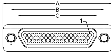
9- 51 contacts: Ø2.24/2.44 (.088/.096) or THD insert 2-56 UNC 2B
