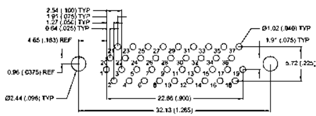
37 CONTACTS - VIEW A
