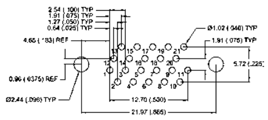
21 CONTACTS - VIEW A
