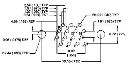
15 CONTACTS - VIEW A
