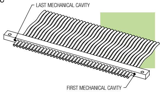
EXAMPLE WITH GUIDE PIN
