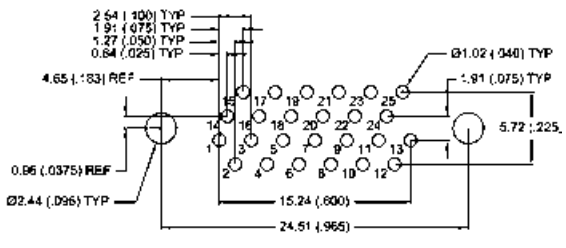
25 CONTACTS - VIEW A
