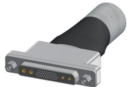
2 POWER COMBO S2.2 + 2 COAXIAL COMBO S3 CONTACTS + 40 SIGNALS, INTEGRATED IN A HARNESS
