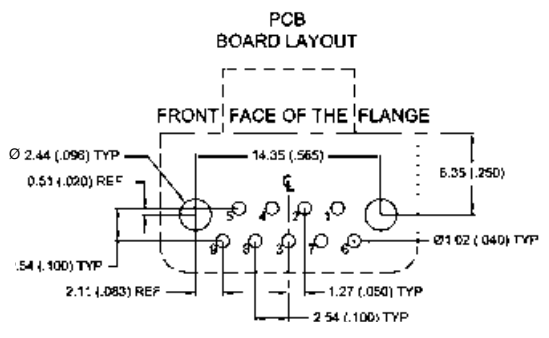
9 CONTACTS - VIEW B
