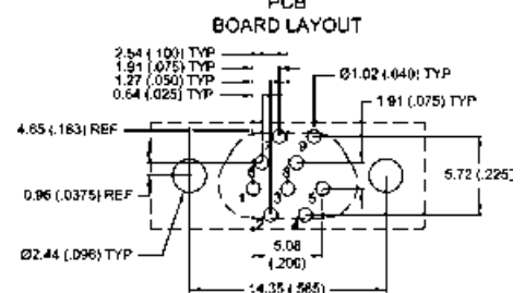
9 CONTACTS - VIEW A
