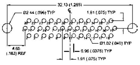
37 CONTACTS - VIEW A
