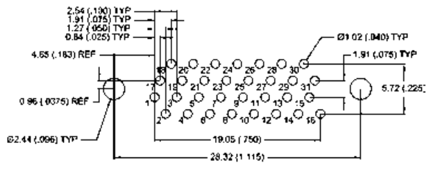
31 CONTACTS - VIEW A
