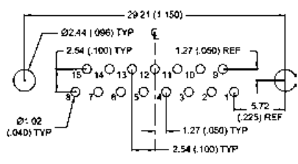
15 CONTACTS - VIEW A
