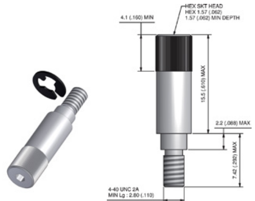
KIT PART NUMBER: MDAHM513 According to M83513/05-13 Hardware code: N
