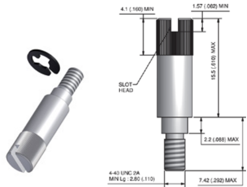
KIT PART NUMBER: MDAHM516 According to M83513/05-16 Hardware code: T
